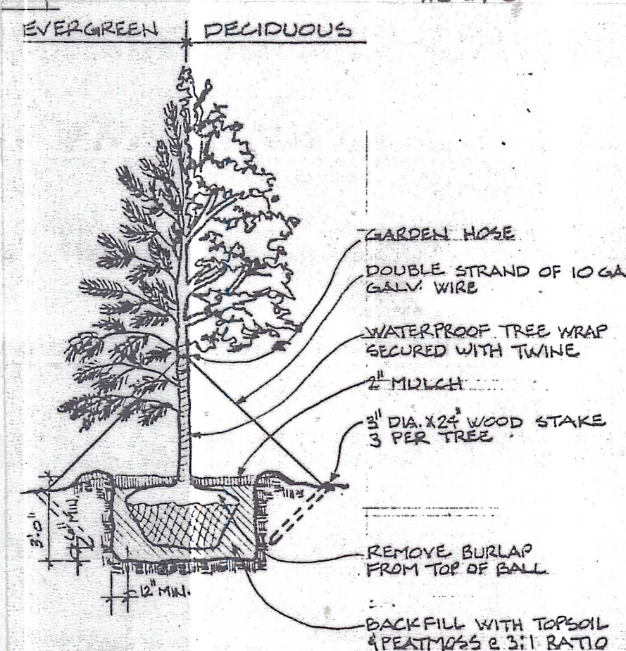
TREE DETAIL
