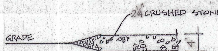
ANTI-TRACKING APRON
